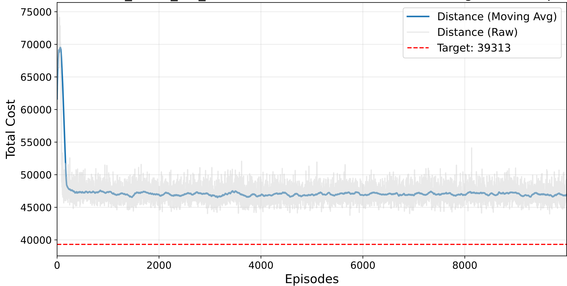
Final NO_MASK_NO_BAYESIAN Masked AutoRL-SOP Training - ft70.1.sop
